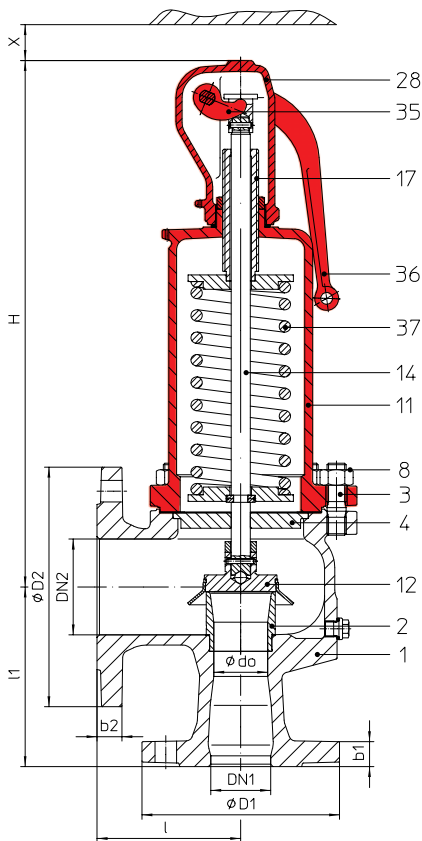
Fig. ... .901 closed lifting device closed bonnet
