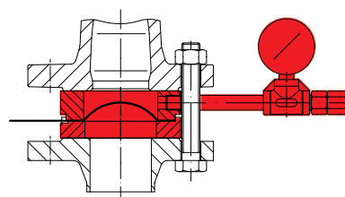
Rupture disc
