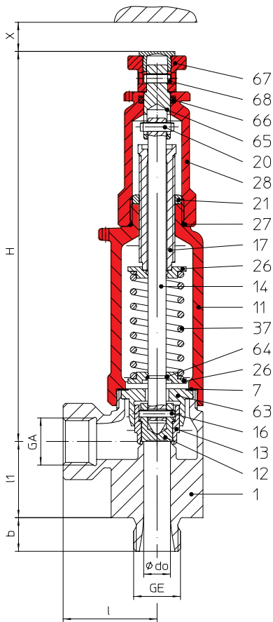
Fig. 67 .951 closed lifting device
