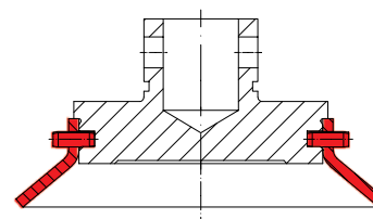
Removable lifting aid Chemical-execution
