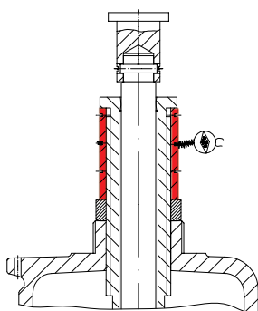
Lock bush
