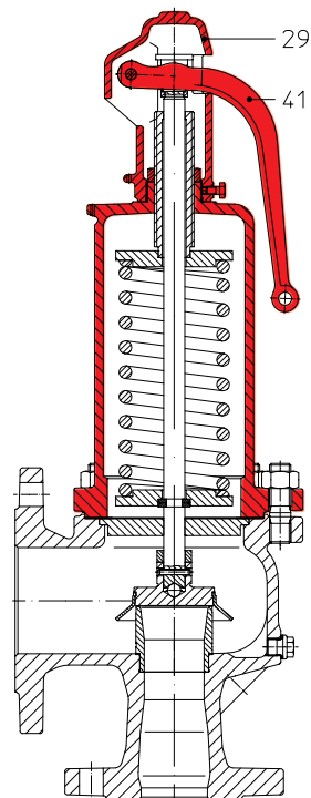
Fig. ... .912 open lifting device closed bonnet
