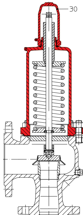
Fig. ... .911 gastight cap closed bonnet
