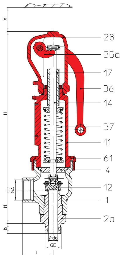
Fig. 25.941 closed lifting device
